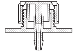
DEBİ AYARLI HAT ÜSTÜ DAMLATICI FLOW ADJUSTABLE ON - LINE DRIPPERS
